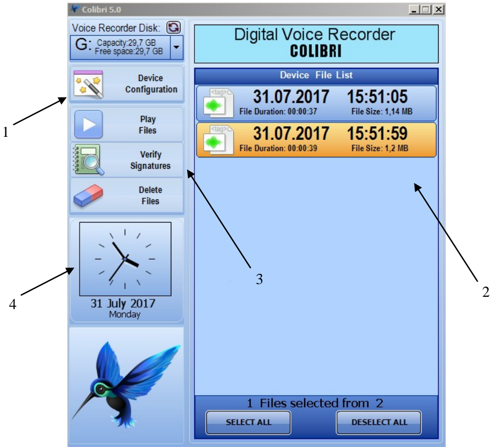
Figure 6. Colibri.exe Program
